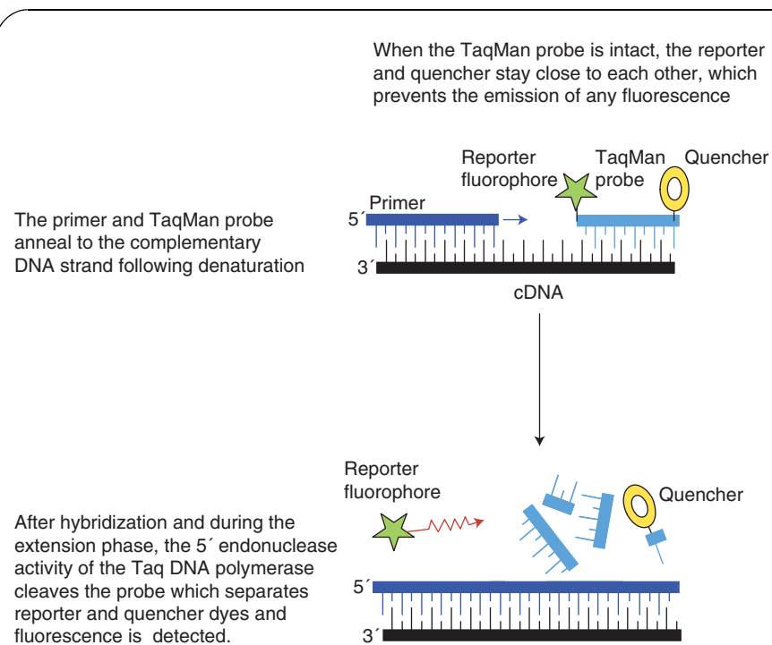
Figure 1. Hydrolysis probes (e.g., TaqMan assay).
